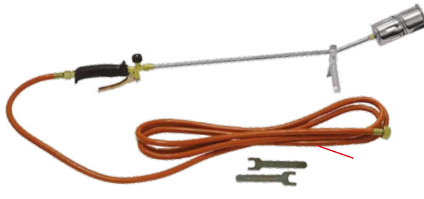
Brazing tool kit nozzle 60 mm, 58kW
